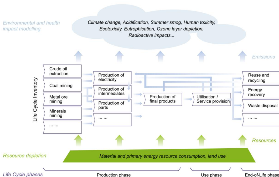
Fig. 1. Scheme of a product’s life cycle along the supply chain of production, the product’s use and disposal, as well as the related impact topics.
